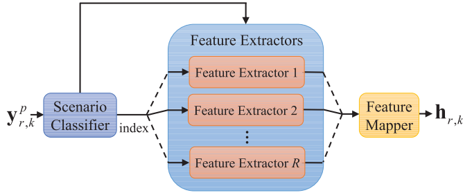
Fig. 3. The proposed hierarchical downlink channel estimation network.
